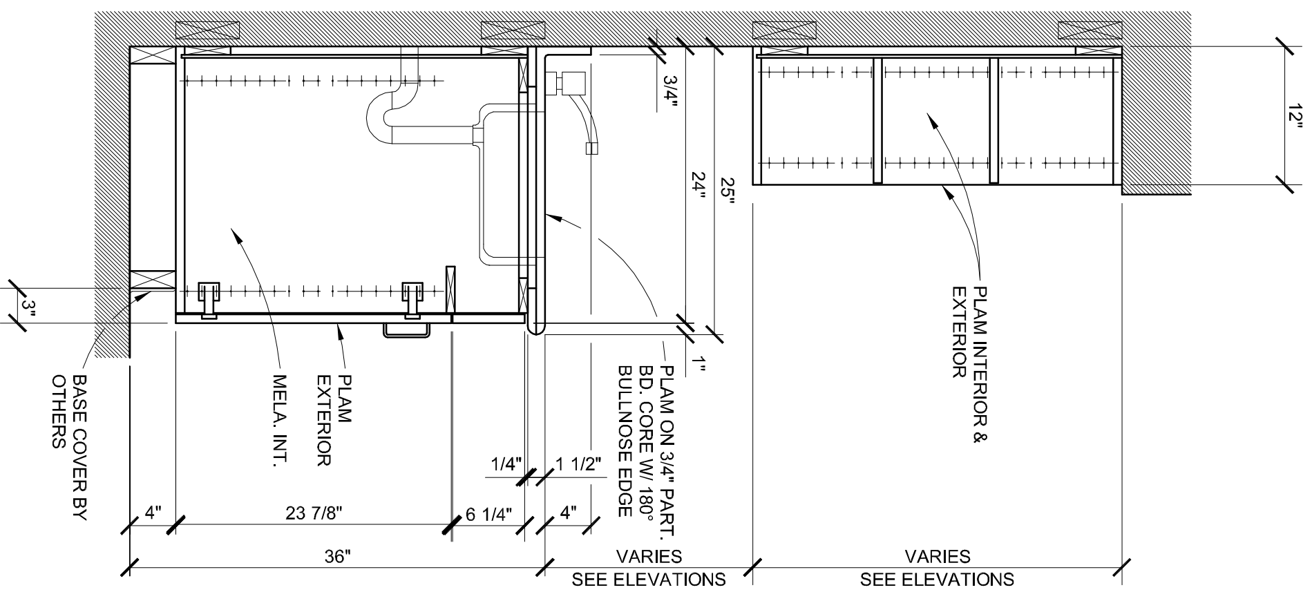
E SECTION THRU WALL & SINK BASE CABTS.
