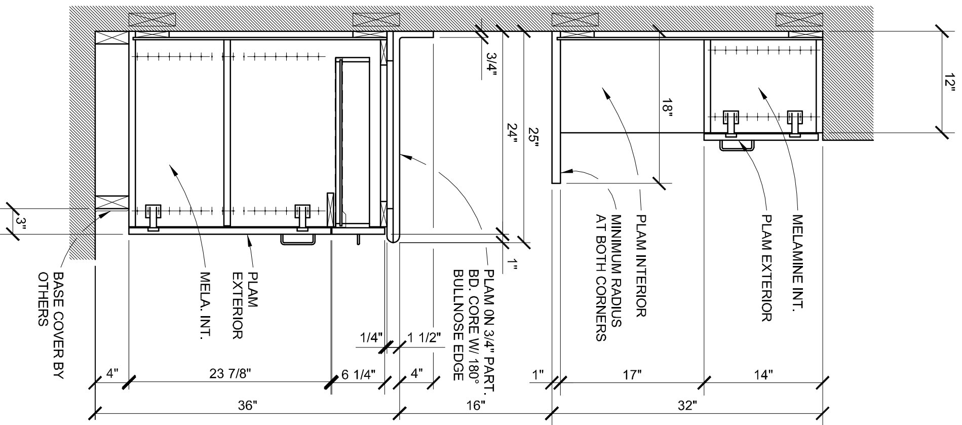
D SECTION THRU MICROWAVE & BASE CABTS.
