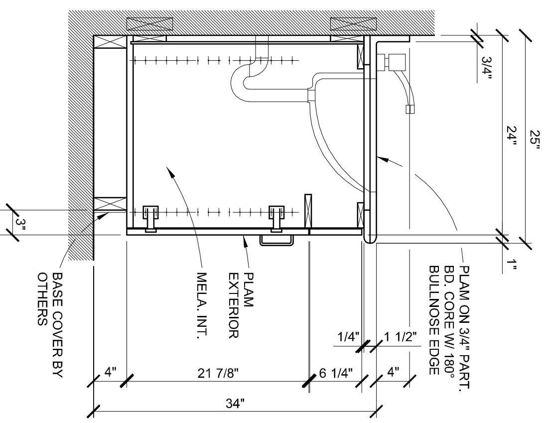
F SECTION THRU SINK BASE CABINET
