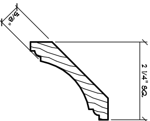
M11 CROWN MOULD 5/8" x 3 3/16"
