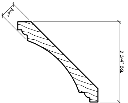
M4 CROWN MOULD 3 3/4" x 3 3/4"
