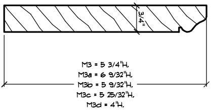
M3 BASE & RAIL 3/4" x 1 LGH.
