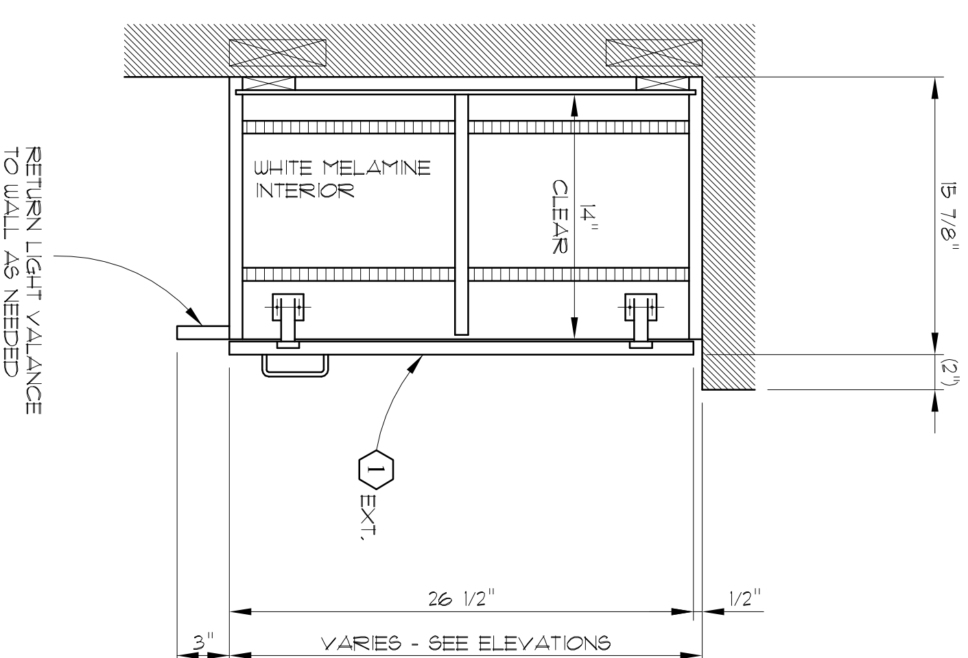
SECTION H SECTION THRU WALL CABINET SCALE: 1 1/2 = 1'-0"
