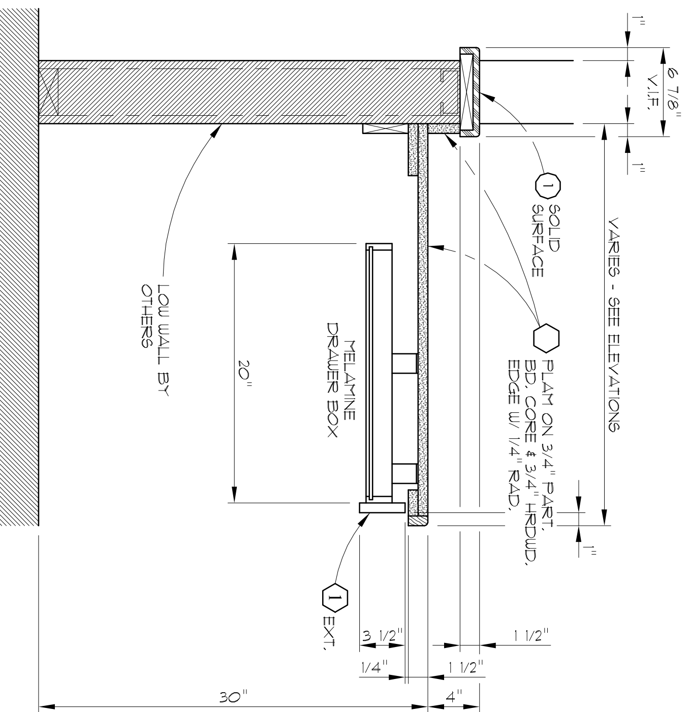
SECTION E SECTION THRU (3) DRAWER BASE CABINET SCALE: 1 1/2 = 1'-0"
