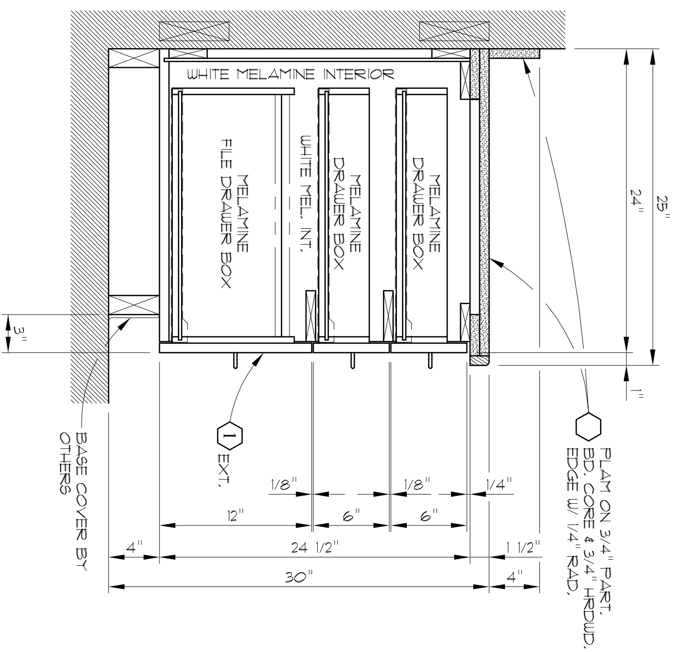
SECTION E SECTION THRU (3) DRAWER BASE CABINET SCALE: 1 1/2 = 1'-0"
