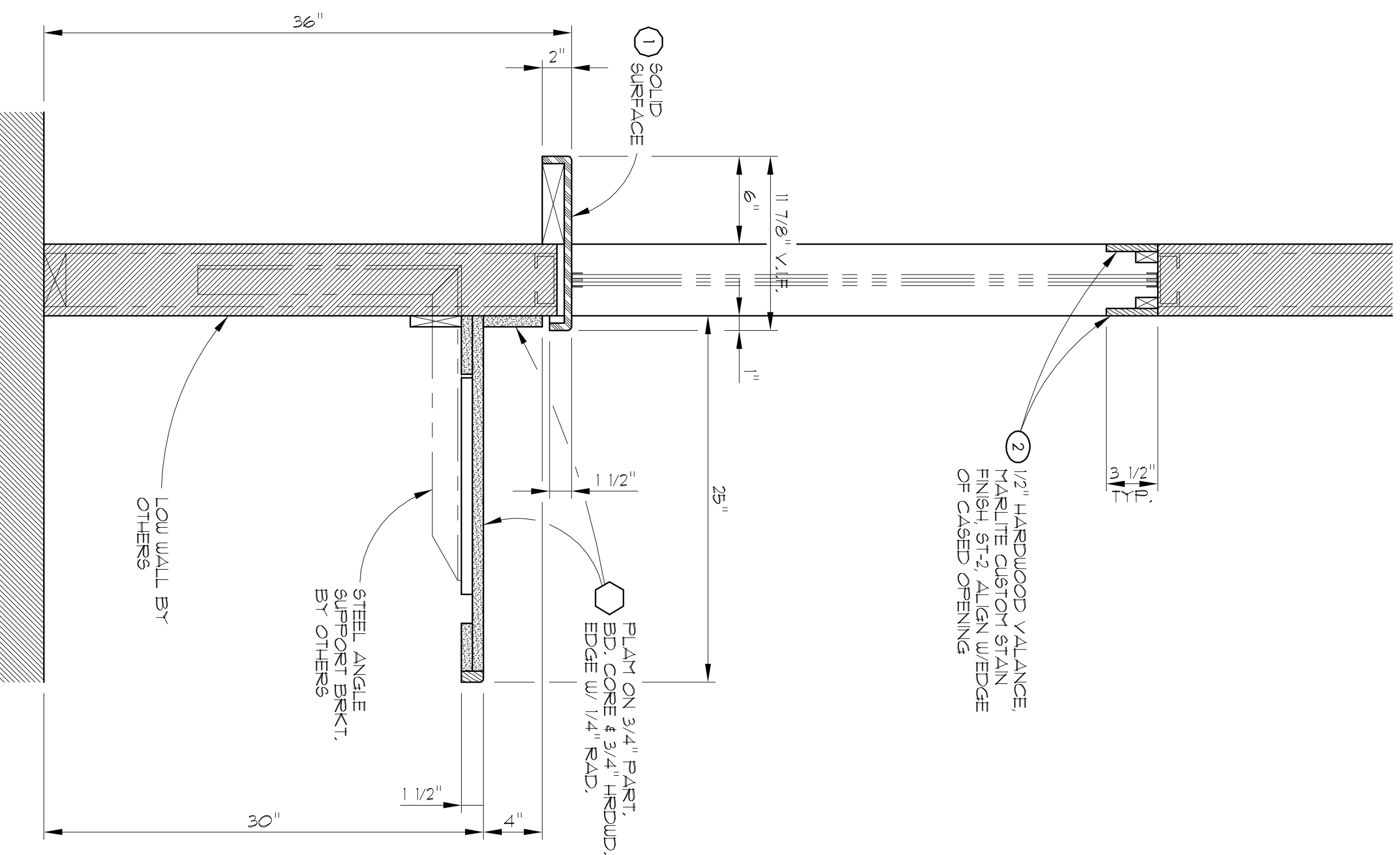
SECTION H SECTION THRU WALL CABINET SCALE: 1 1/2 = 1'-0"
